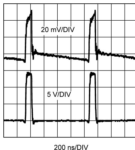
Figure 5. V_{IN} = 14\text{ V} , V_{CC} = 5\text{ V} , V_{OUT} = 1.2\text{ V} , I_{LOAD} = 3.5\text{ A} , f_{SW} = 1\text{ MHz} , 20 MHz Bandwidth Limit
