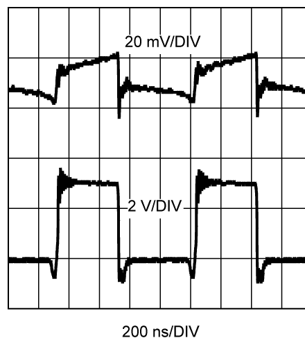
Figure 3. V_{IN} = V_{CC} = 3.3\text{ V} , V_{OUT} = 1.2\text{ V} , I_{LOAD} = 3.5\text{ A} , f_{SW} = 1\text{ MHz} , 20 MHz Bandwidth Limit
