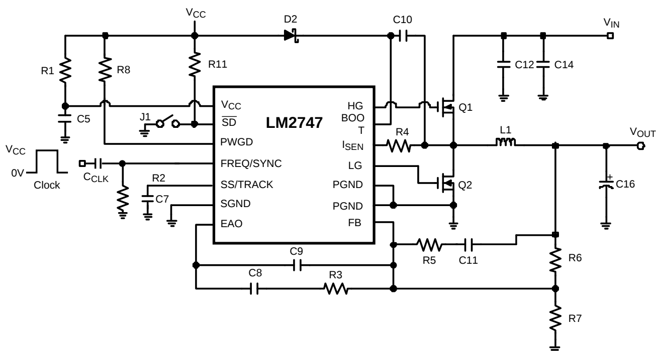
Figure 1. Typical Application
