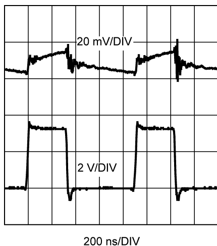
Figure 2. V_{IN} = V_{CC} = 3.3\text{ V} , V_{OUT} = 1.2\text{ V} , I_{LOAD} = 0\text{ A} , f_{SW} = 1\text{ MHz} , 20 MHz Bandwidth Limit
