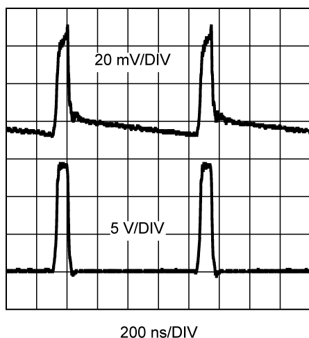
Figure 4. V_{IN} = 14\text{ V} , V_{CC} = 5\text{ V} , V_{OUT} = 1.2\text{ V} , I_{LOAD} = 0\text{ A} , f_{SW} = 1\text{ MHz} , 20 MHz Bandwidth Limit
